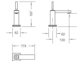
Deck-Mounted LED Basin Mixer JTL9100HG
