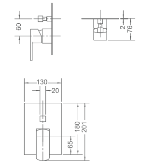
Concealed Shower Mixer with Diverter MXS817960
