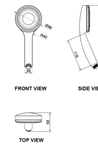
Rain Shower Head HSL429
